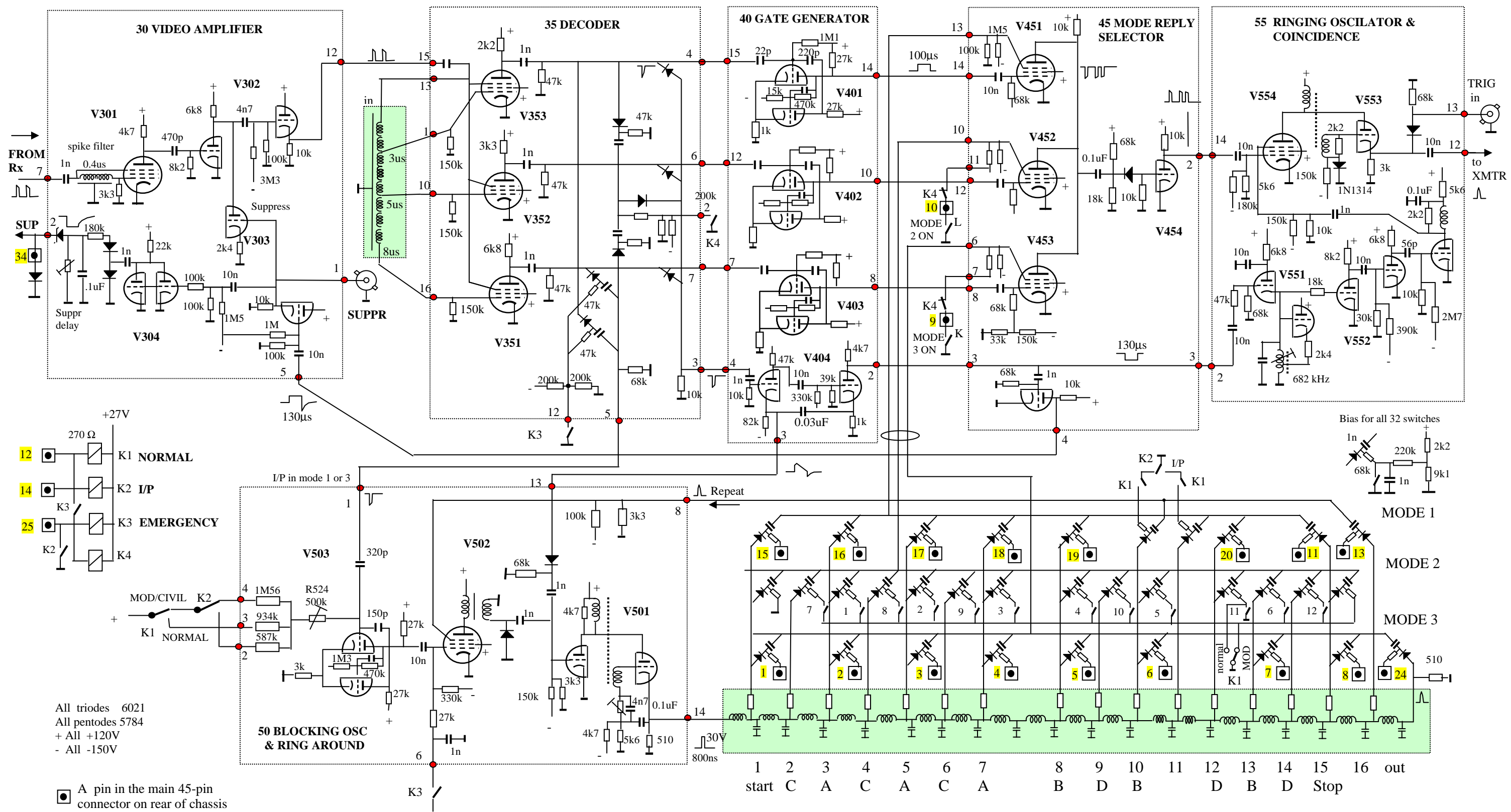
RT 494 - AN / APX44 CODEC Circuit Diagram 15-7-2007
