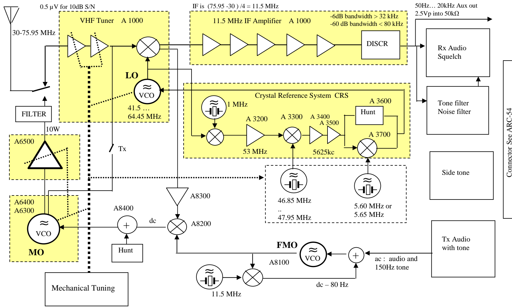
RT-823 / ARC-131 Block Diagram 16-10-2011 kb
