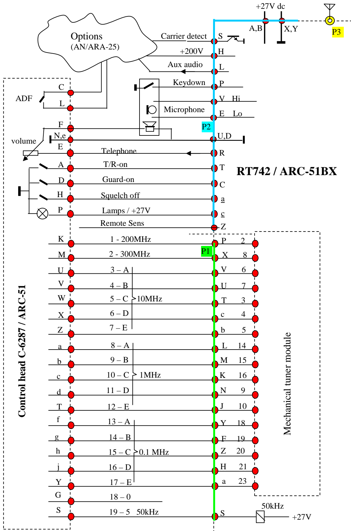
ARC51 External wiring 01-01-2010 kb
