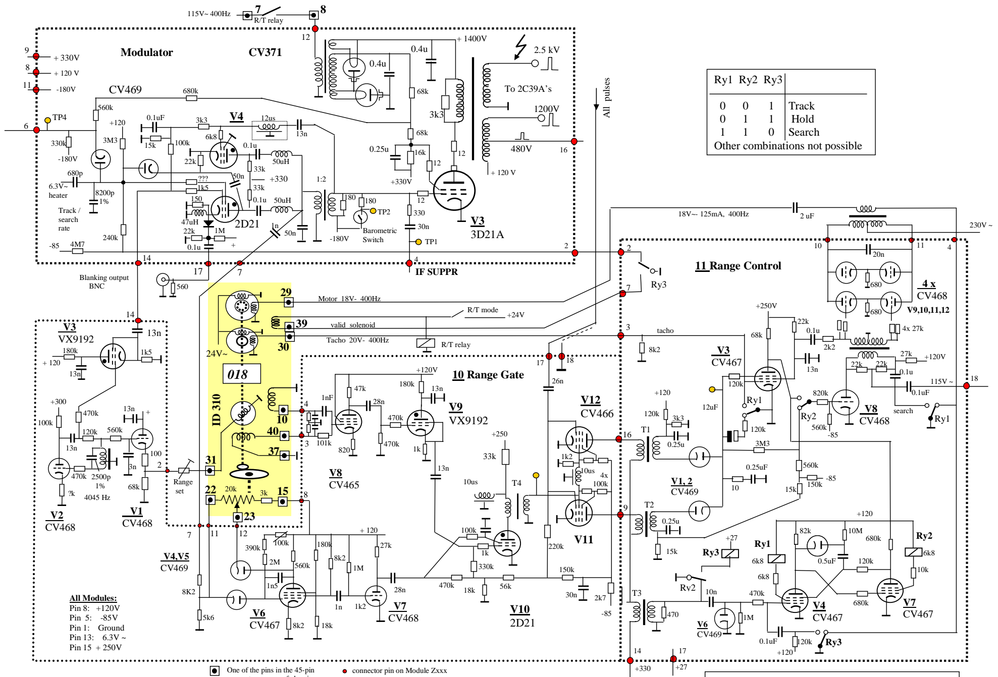
STARN-21 Range Circuits Diagram
